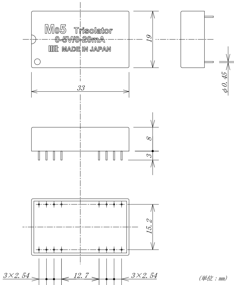
<Pin Assignment>
