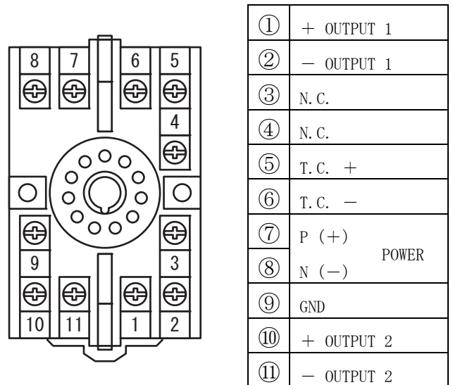
SOKET TOP VIEW
